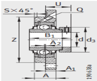
RME、RMEO (到 d = 70 mm)
